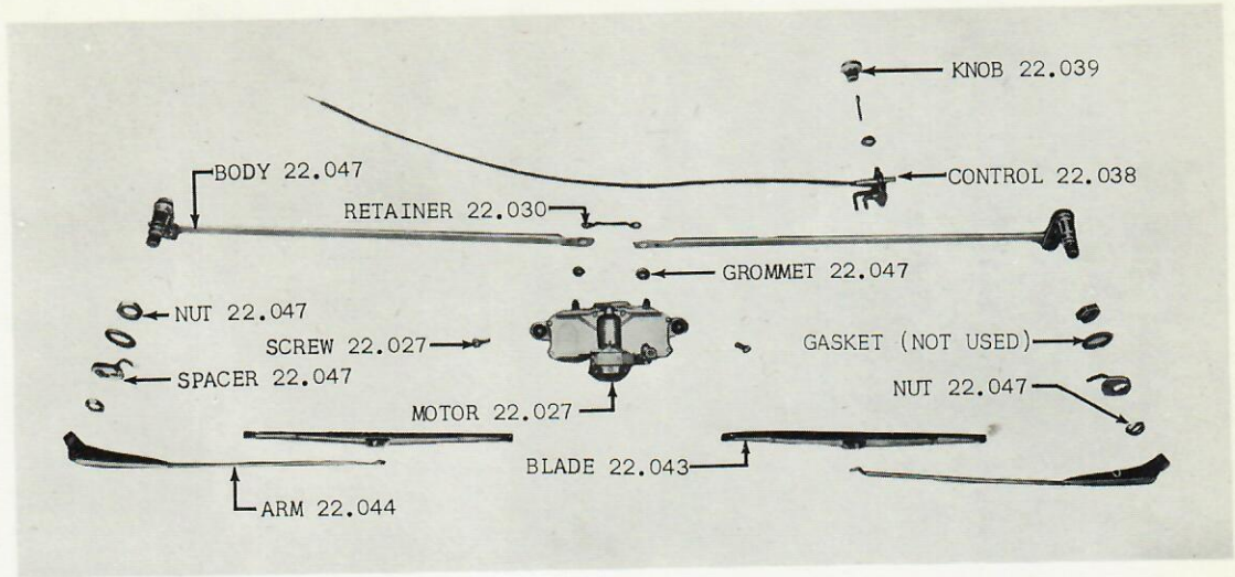
GROUP 22 - FIG. 1 - WINDSHIELD WIPER ASSEMBLY 01-10-20-80
