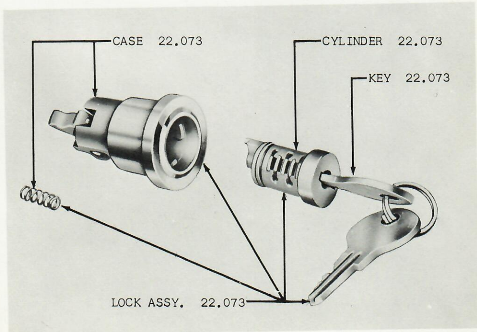
GROUP 22 - FIG. 2 - GLOVE BOX LOCK 01
